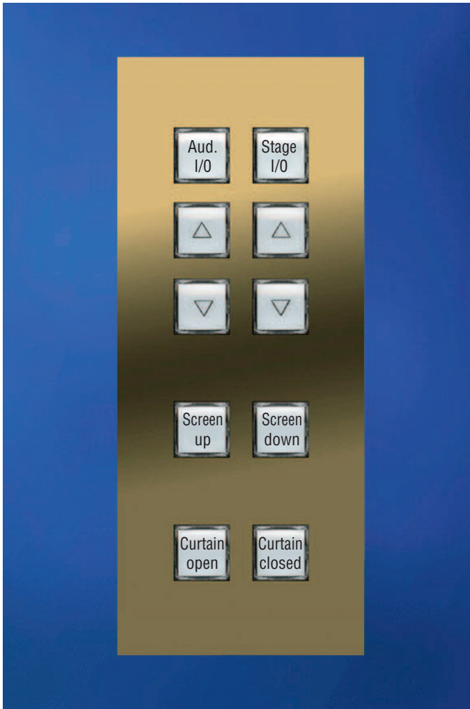
Panel face brass polished with 10 pushbuttons (for e.g. 1 control module type NS2X and 1 module type NS2-SX for AQ dimmers and for electronic ballasts or transformers with 1-10V interface, additionally with 1 pushbutton 'UP' and 'DOWN' for screens or curtains).
