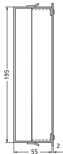
wall-recessed housing, side view
