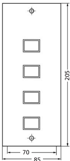
Panel face
